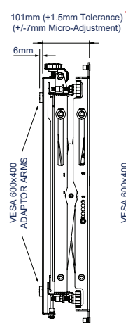
SIDE VIEW CLOSED
