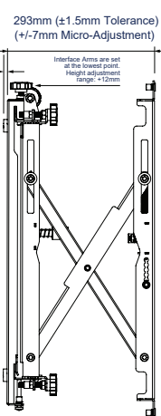
SIDE VIEW EXTENDED
