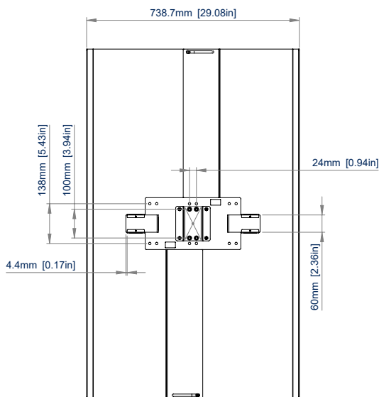
FRONT VIEW MAXIMUM WIDTH
