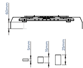
SPACERS
